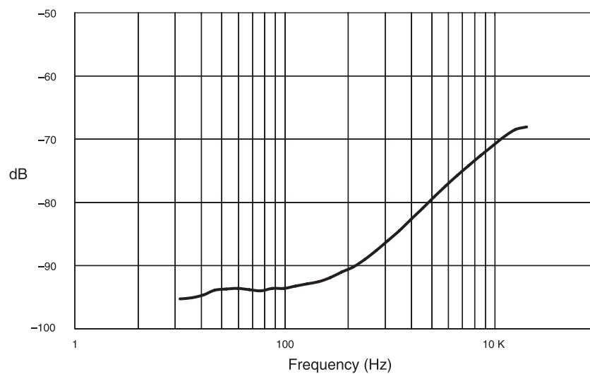
Figure 7.7 CTs 8200 Typical Crosstalk vs. Frequency
